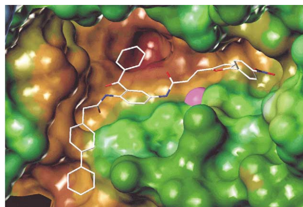
Figure 4. Docking solution of the biphenyl substituted inhibitor 4u showing the biphenyl residue in a lipophilic channel which normally harbours the farnesyl residue of the farnesylated protein.
