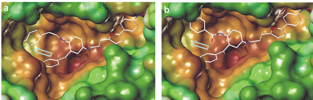
Figure 1. Docking solution of inhibitors 4f (a) and 4a (b) showing the terminal aryl of 4f in a binding pocket (indicated by a blue arrow) while the phenyl residue of 4a does not reach into this pocket.
