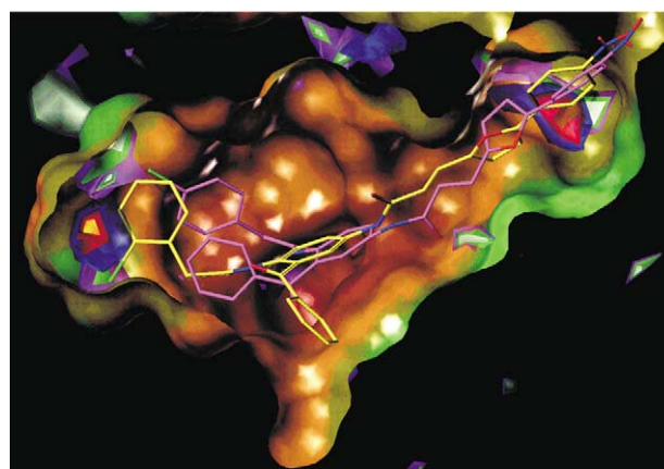
Figure 3. Comparison of the docking solutions of the para bromo substituted inhibitor 4k (magenta) and the ortho bromo substituted inhibitor 4l (yellow). Areas which according to DrugScore prevalently bind hydrogen bond acceptors are indicated by a violet-green-white cloud (increasing prevalence). It is clearly visible that the ortho bromo substituent points to such an area while the para bromo substituent cannot reach such an area.
