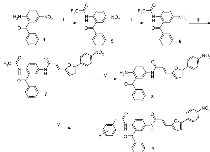
Scheme 2. (I) TFAA, DCM/pyridine, 0 °C, 2 h; (II) \text{SnCl}_2 \times 2\text{H}_2\text{O} , EtOAc, reflux 2 h; (III) 3-[5-(4-nitrophenyl)-2-furyl]acrylic acid chloride, toluene/dioxane, reflux, 2 h; (IV) \text{K}_2\text{CO}_3 , dioxane/ \text{H}_2\text{O} , reflux, 3 h; (V) R\text{-C}_6\text{H}_4\text{-CH}_2\text{-COCl} , toluene/dioxane, reflux, 2 h.
