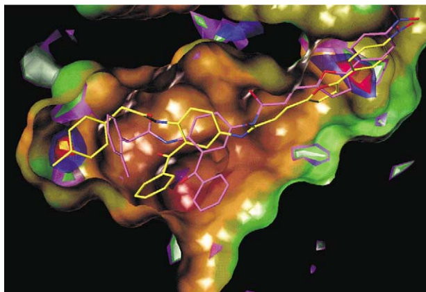
Figure 2. Comparison of the docking solutions of the para methyl substituted inhibitor 4f (yellow) and the ortho methyl substituted inhibitor 4h (magenta). Areas which according to DrugScore prevalently bind methyl are indicated by a blue-yellow-red cloud (increasing prevalence). The para methyl group of inhibitor 4f (yellow) is located in such an area while the ortho methyl group of 4h (magenta) is directed in no such region.
