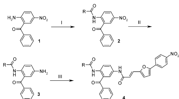
Scheme 1. (I) R\text{-CO-Cl} , toluene/dioxane, reflux, 2 h; (II) \text{SnCl}_2 \times 2\text{H}_2\text{O} , EtOAc, reflux 2 h; (III) 3-[5-(4-nitrophenyl)-2-furyl]acrylic acid chloride, toluene/dioxane, reflux, 2 h.
